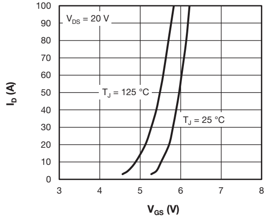
Fig. 7 - Typical MOSFET Transfer Characteristics
