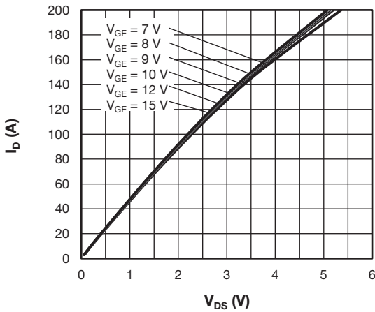
Fig. 4 - Typical MOSFET Output Characteristics, at T_J = 125^\circ\text{C}
