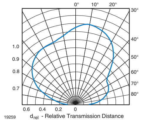
Fig. 5 - Vertical Directivity
