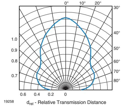
Fig. 4 - Horizontal Directivity
