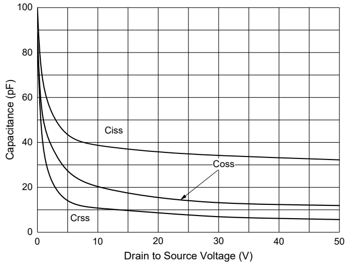
Fig. 7 - Capacitance Characteristics
