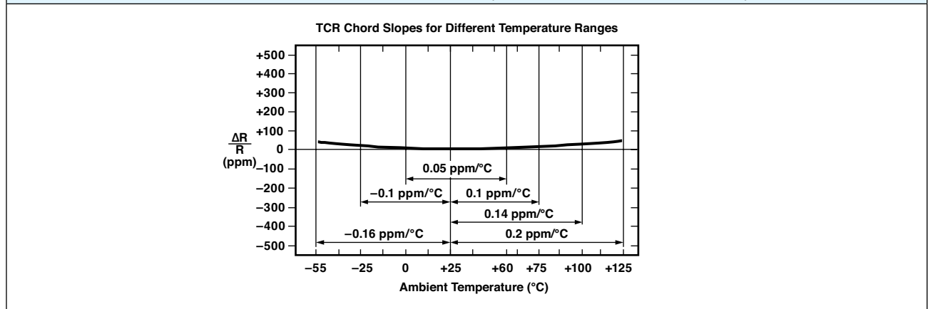
Figure 4 – Typical Resistance/Temperature Curve (for more details, see Table 1A)
