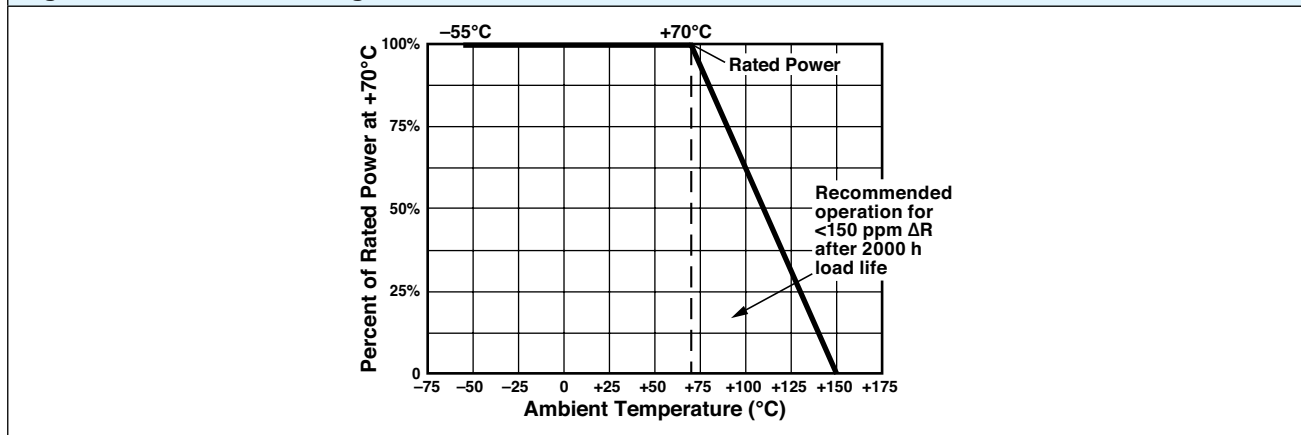
Figure 3 – Power Derating Curve
