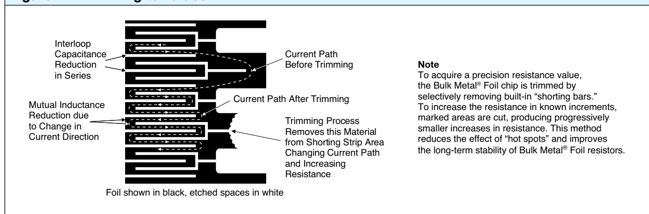
Figure 1 – Trimming to Values
